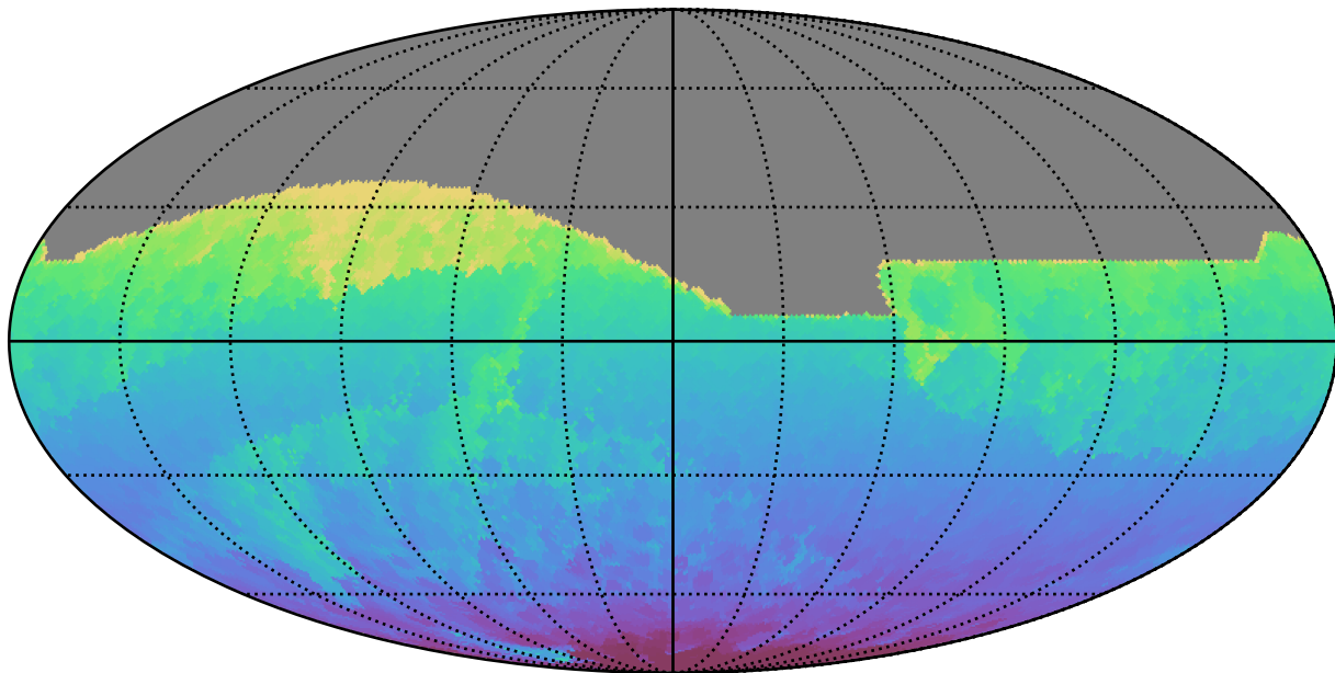
ddf_loaded_fl1_v3.4_10yrs All sky all bands: Min HA
