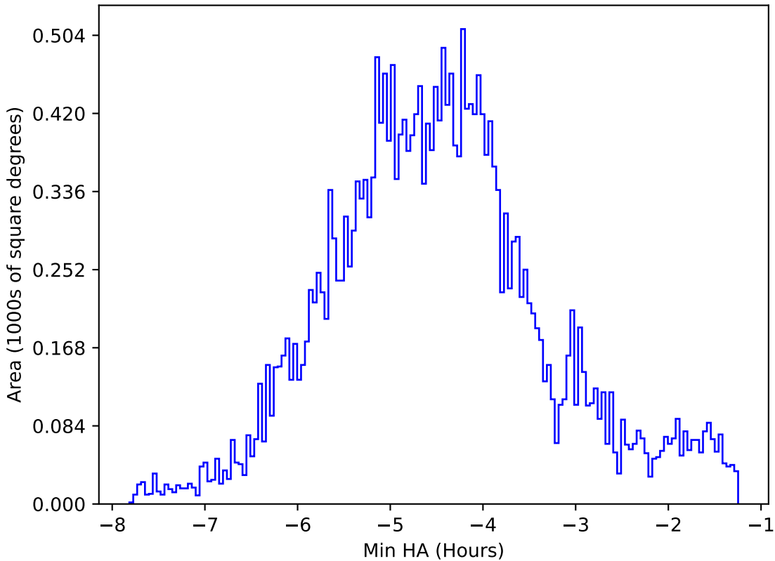
ddf_loaded_fl1_v3.4_10yrs All sky all bands: Min HA
