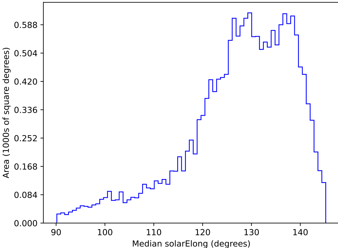
ddf_loaded_fl1_v3.4_10yrs WFD z band: Median solarElong
