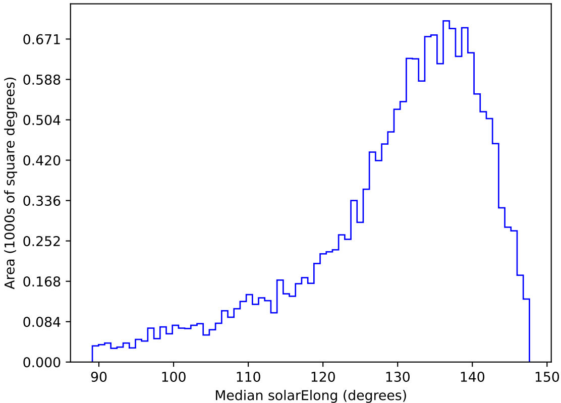
ddf_loaded_fl1_v3.4_10yrs WFD y band: Median solarElong
