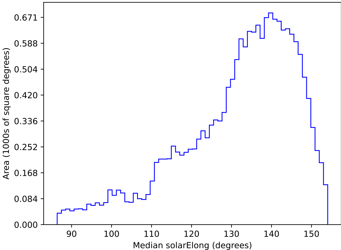
ddf_loaded_fl1_v3.4_10yrs WFD u band: Median solarElong
