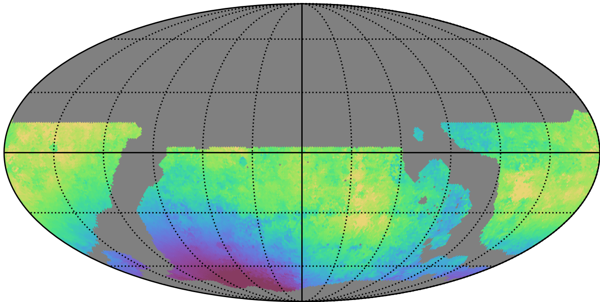
ddf_loaded_fl1_v3.4_10yrs WFD g band: Median solarElong
