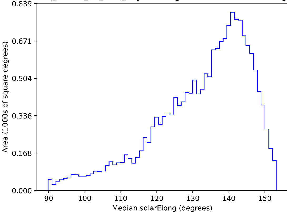
ddf_loaded_fl1_v3.4_10yrs WFD g band: Median solarElong
