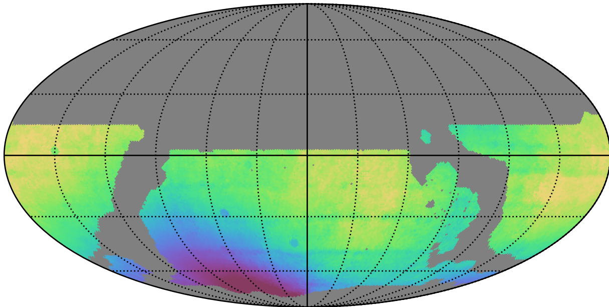
ddf_loaded_fl1_v3.4_10yrs WFD all bands: Median solarElong
