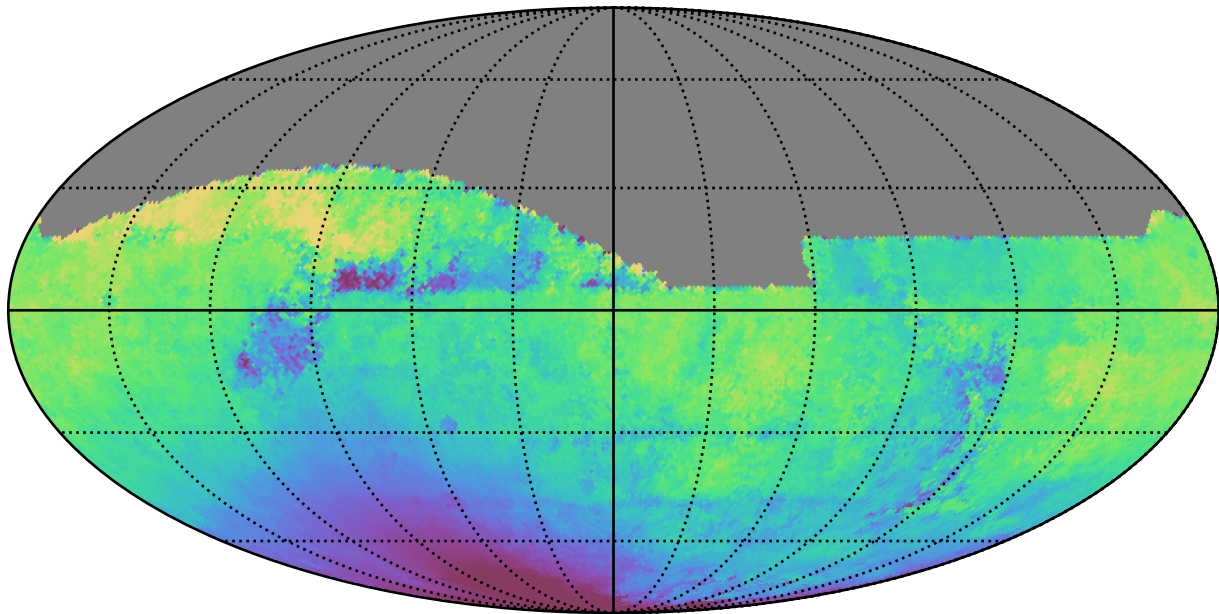
ddf_loaded_fl1_v3.4_10yrs All sky z band: Median solarElong
