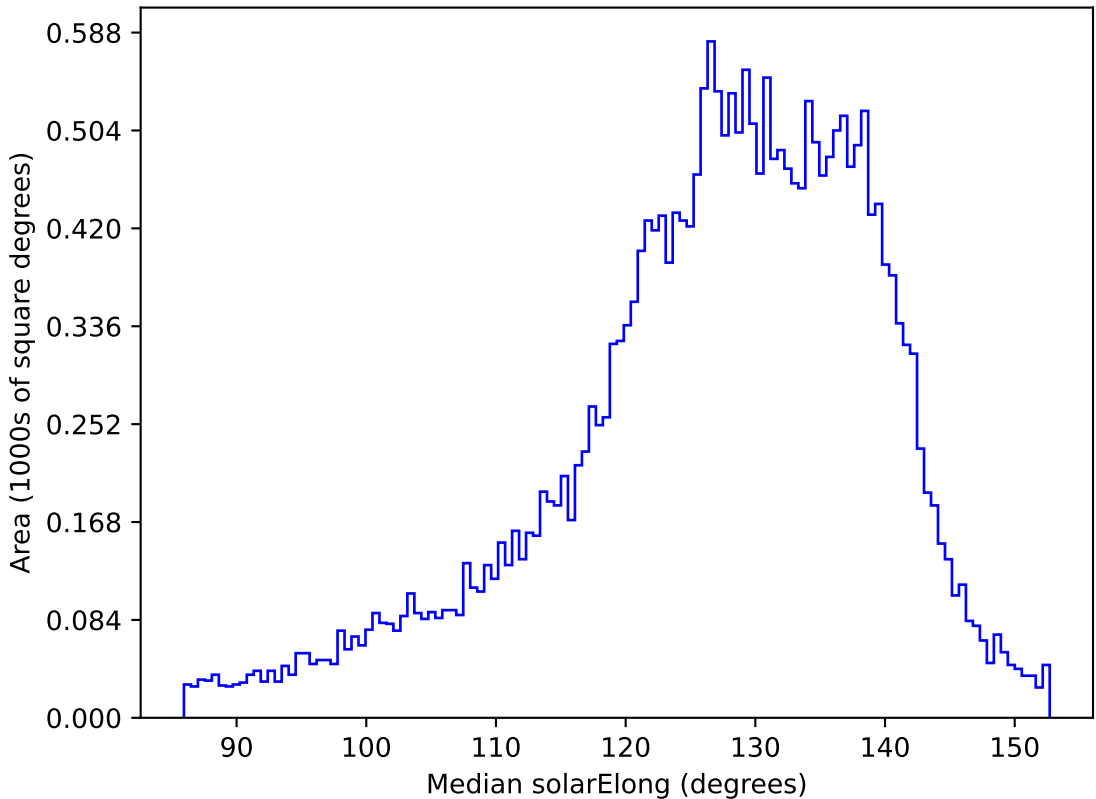
ddf_loaded_fl1_v3.4_10yrs All sky z band: Median solarElong
