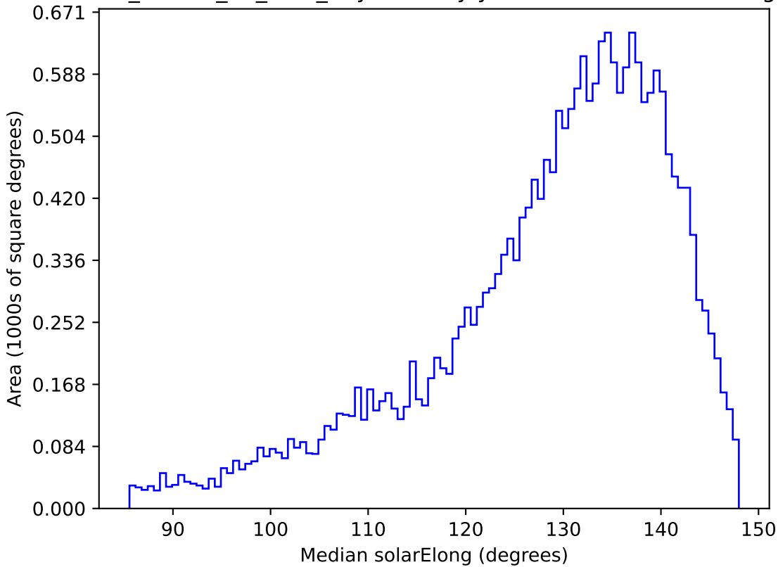
ddf_loaded_fl1_v3.4_10yrs All sky y band: Median solarElong
