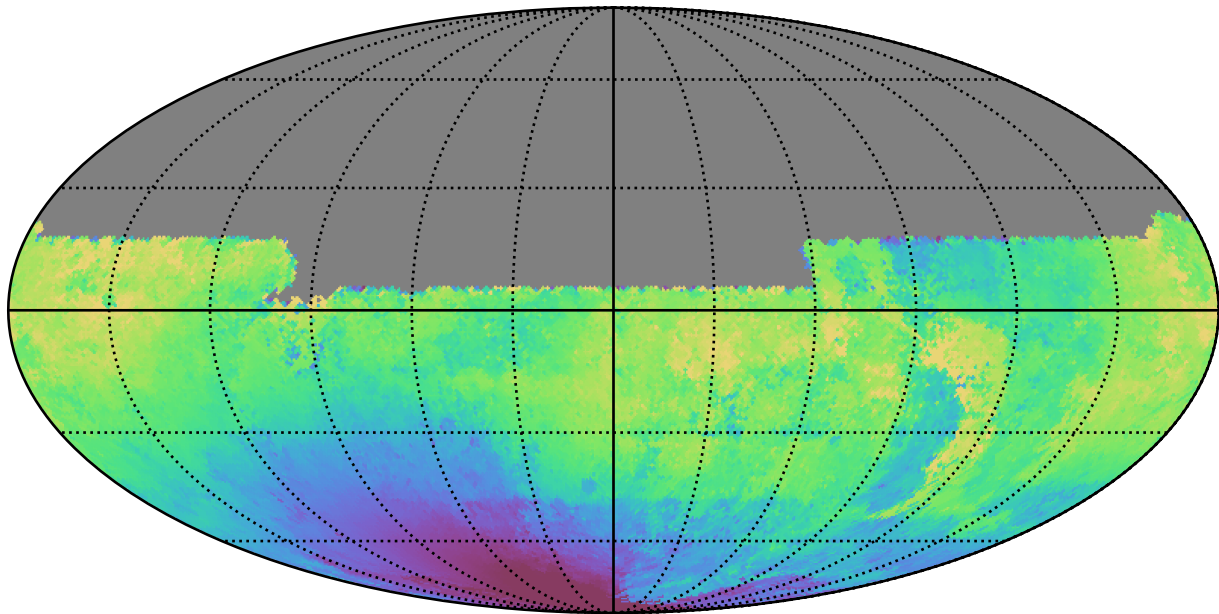
ddf_loaded_fl1_v3.4_10yrs All sky u band: Median solarElong
