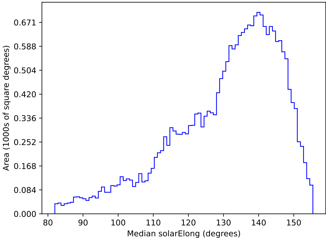
ddf_loaded_fl1_v3.4_10yrs All sky u band: Median solarElong
