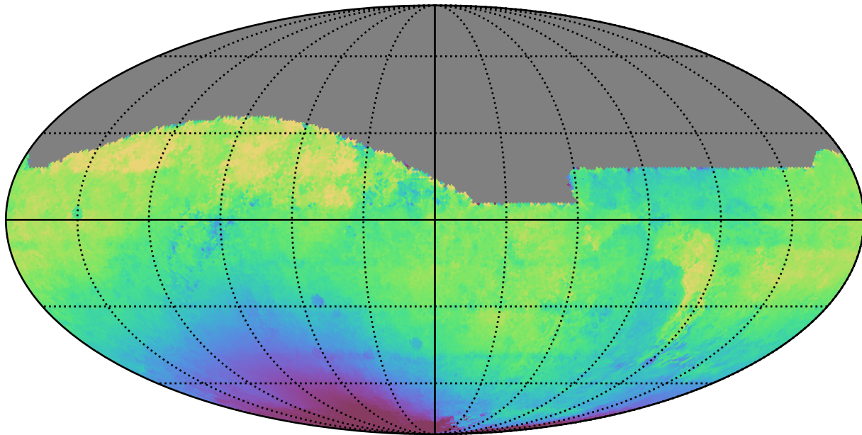
ddf_loaded_fl1_v3.4_10yrs All sky r band: Median solarElong
