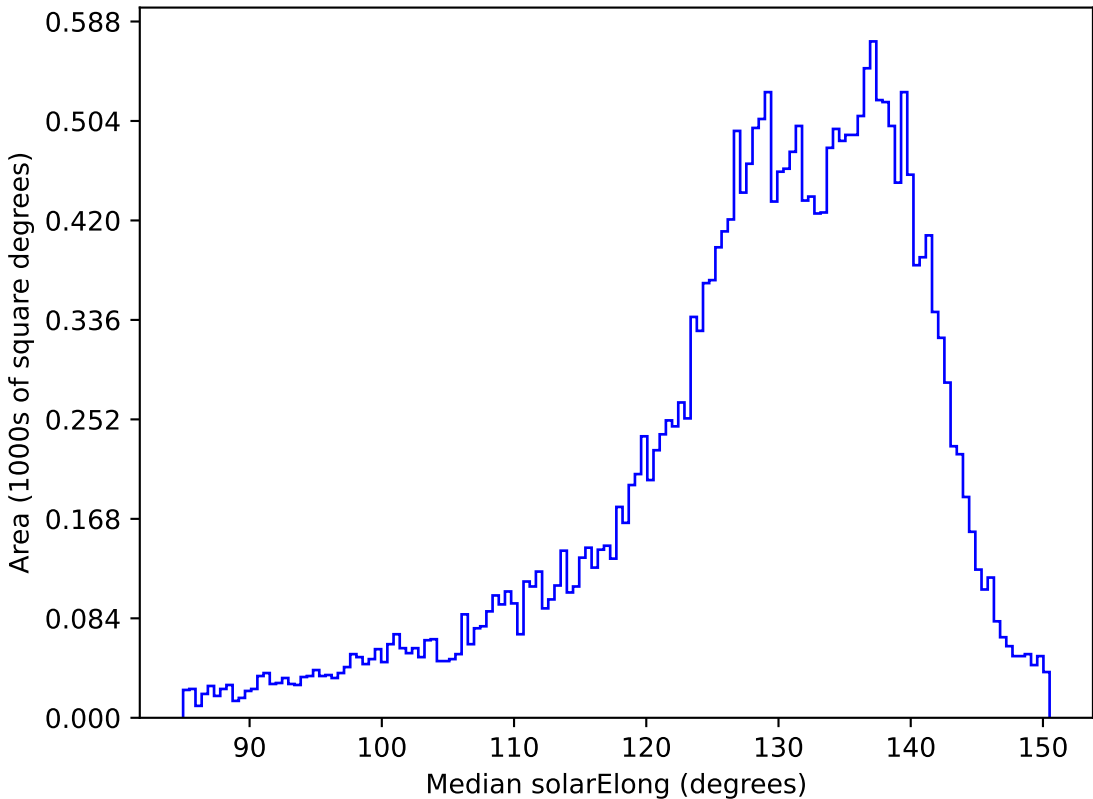
ddf_loaded_fl1_v3.4_10yrs All sky i band: Median solarElong
