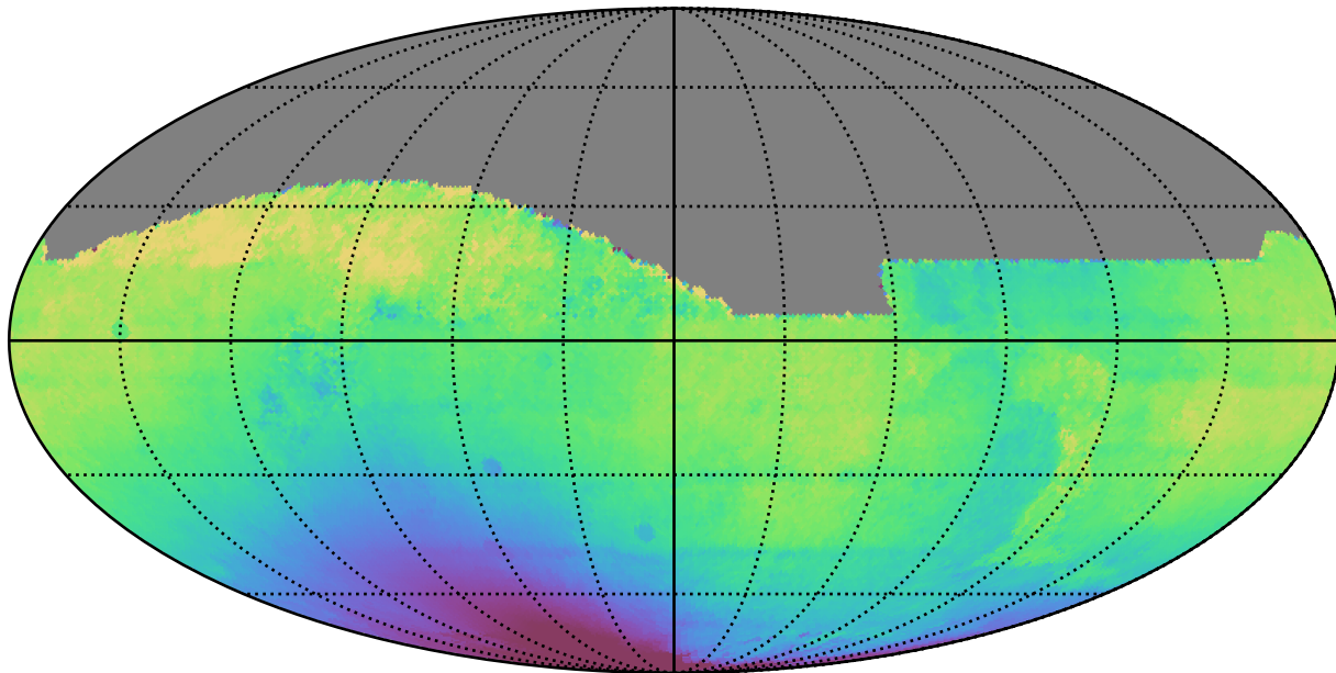
ddf_loaded_fl1_v3.4_10yrs All sky all bands: Median solarElong
