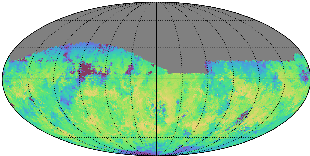
ddf_loaded_fl1_v3.4_10yrs Yr 1 z band: Median skyBrightness
