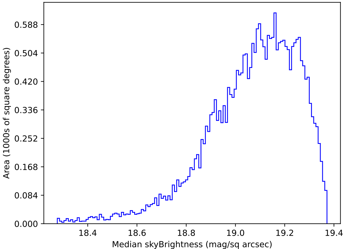
ddf_loaded_fl1_v3.4_10yrs Yr 1 z band: Median skyBrightness
