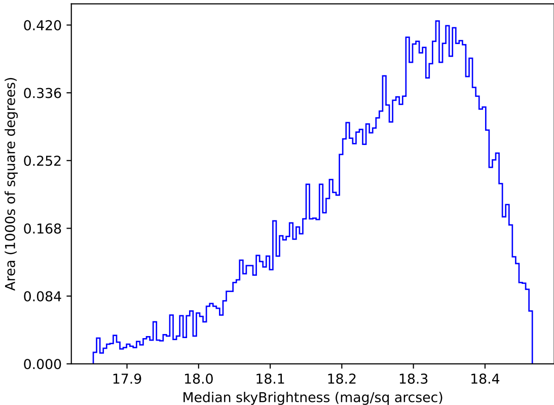
ddf_loaded_fl1_v3.4_10yrs Yr 1 y band: Median skyBrightness
