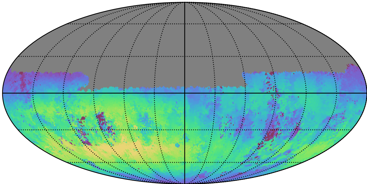
ddf_loaded_fl1_v3.4_10yrs Yr 1 u band: Median skyBrightness
