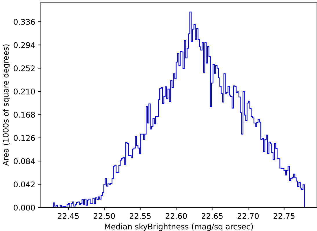
ddf_loaded_fl1_v3.4_10yrs Yr 1 u band: Median skyBrightness
