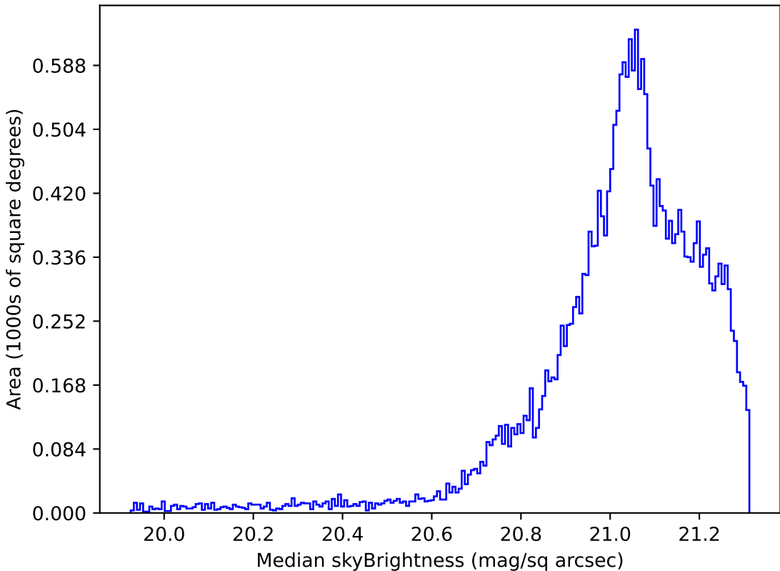
ddf_loaded_fl1_v3.4_10yrs Yr 1 r band: Median skyBrightness
