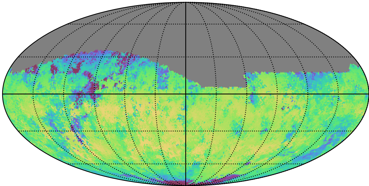
ddf_loaded_fl1_v3.4_10yrs Yr 1 i band: Median skyBrightness
