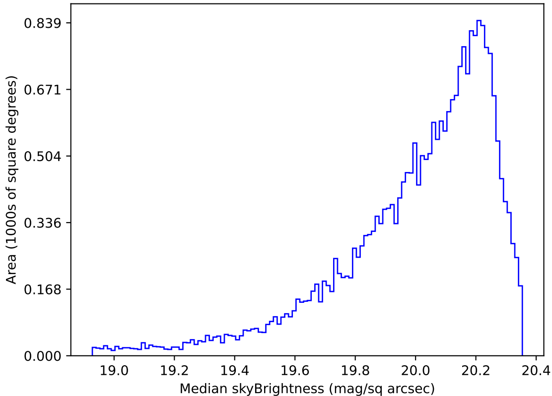
ddf_loaded_fl1_v3.4_10yrs Yr 1 i band: Median skyBrightness
