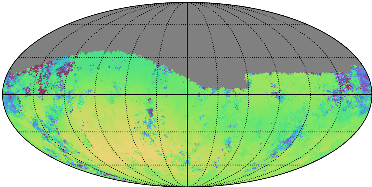
ddf_loaded_fl1_v3.4_10yrs Yr 1 g band: Median skyBrightness
