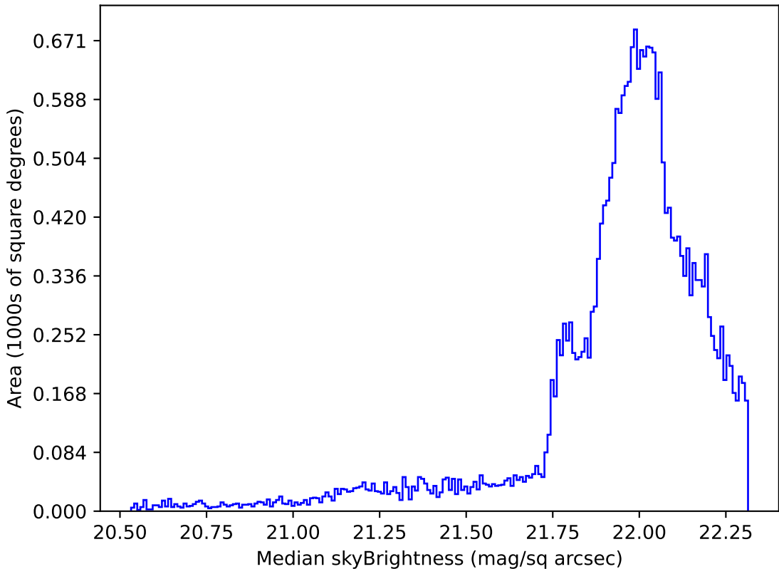
ddf_loaded_fl1_v3.4_10yrs Yr 1 g band: Median skyBrightness
