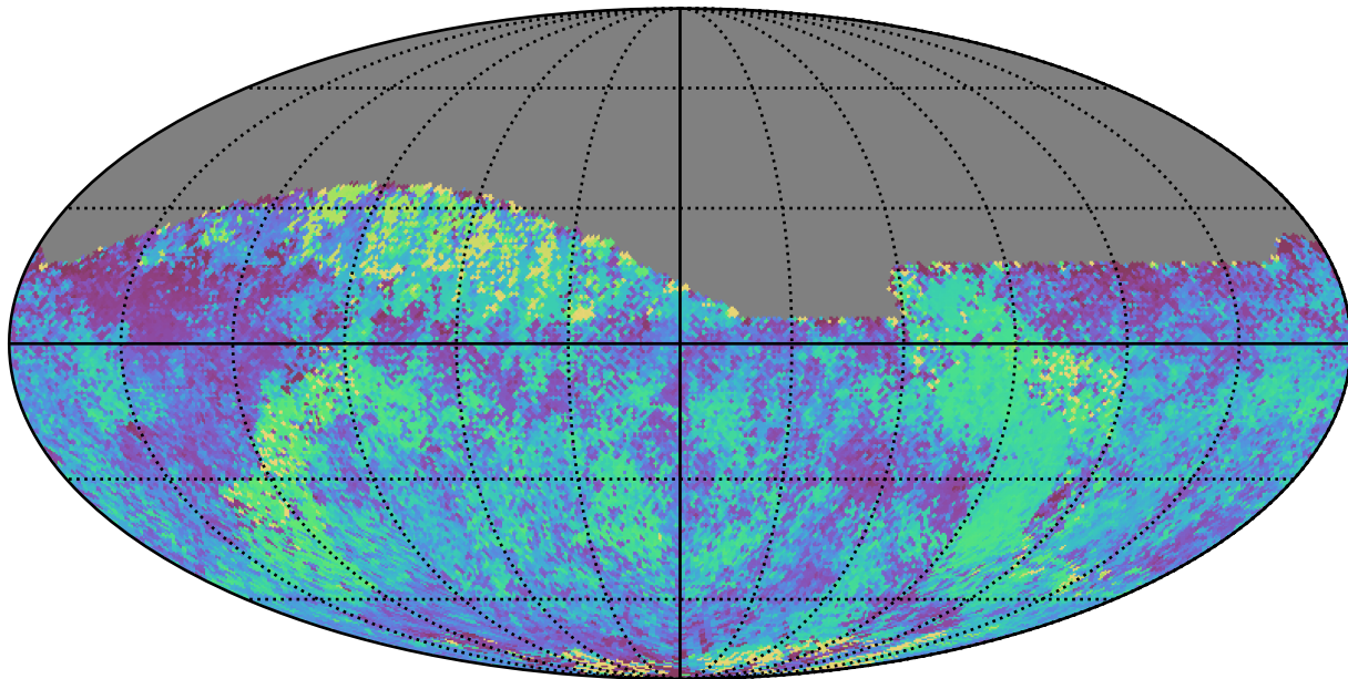
ddf_loaded_fl1_v3.4_10yrs Yr 1 all bands: Median skyBrightness
