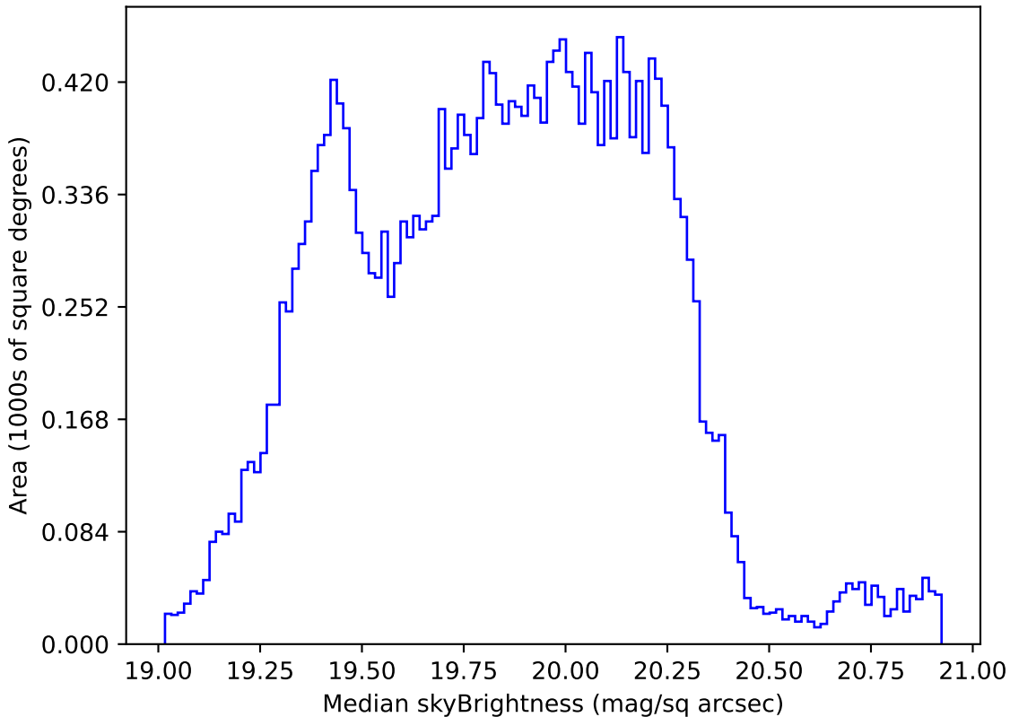
ddf_loaded_fl1_v3.4_10yrs Yr 1 all bands: Median skyBrightness
