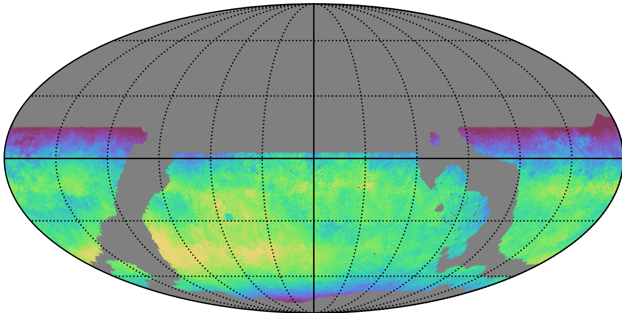
ddf_loaded_fl1_v3.4_10yrs WFD y band: Median skyBrightness
