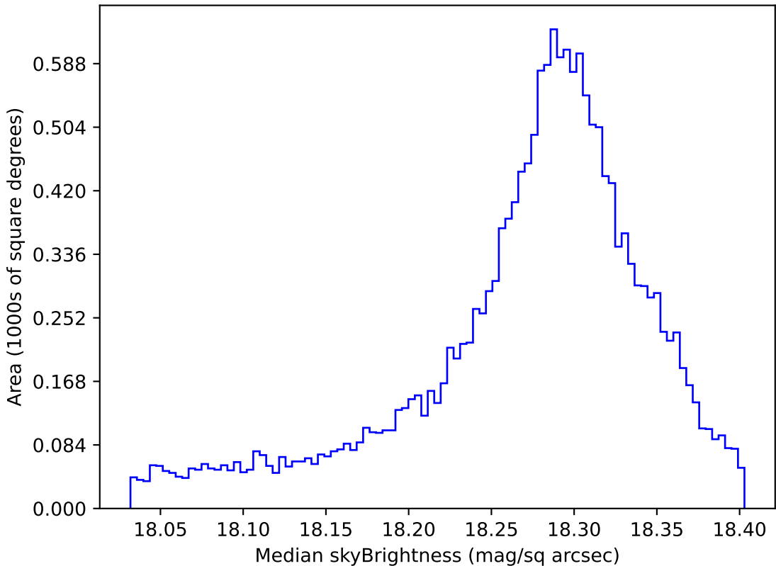
ddf_loaded_fl1_v3.4_10yrs WFD y band: Median skyBrightness
