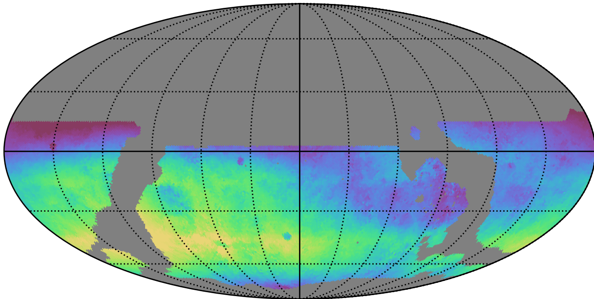
ddf_loaded_fl1_v3.4_10yrs WFD u band: Median skyBrightness
