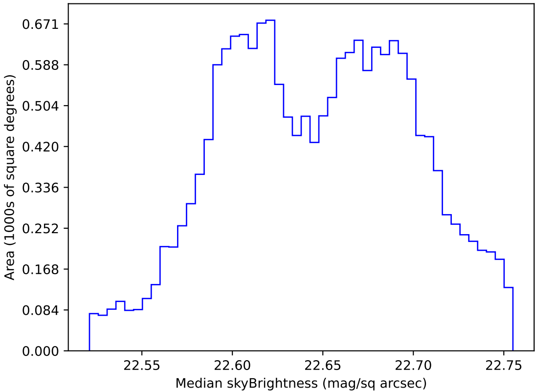
ddf_loaded_fl1_v3.4_10yrs WFD u band: Median skyBrightness
