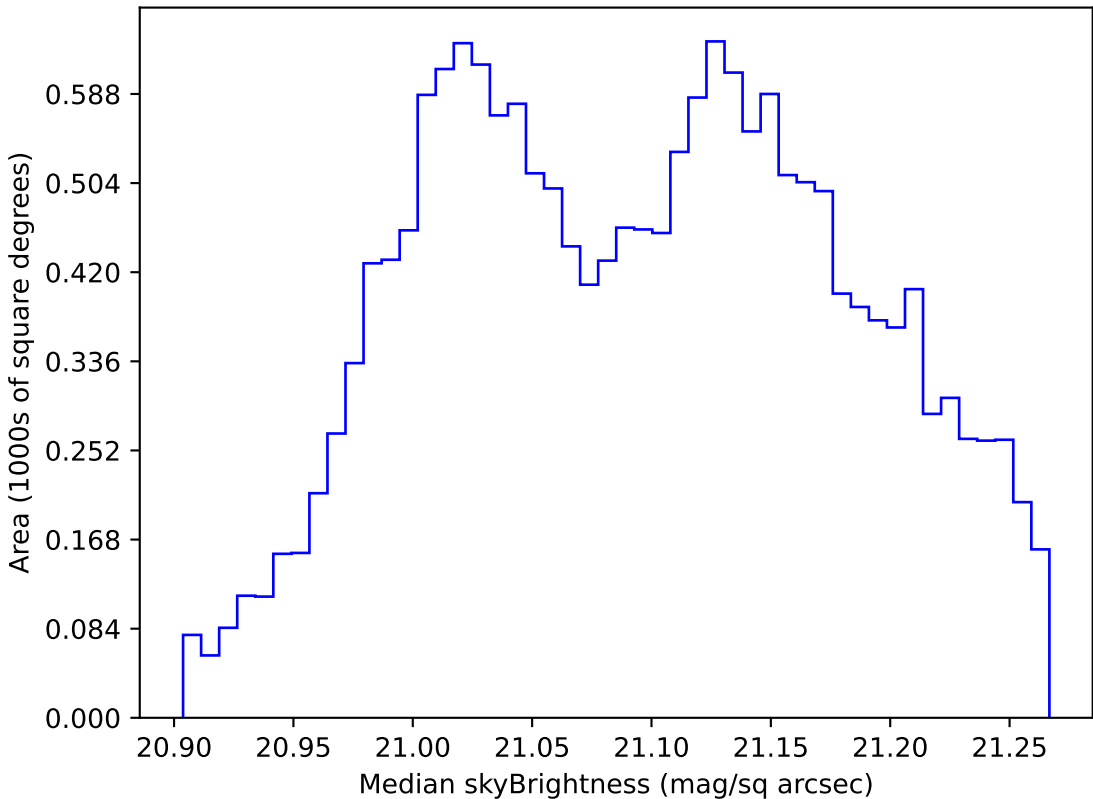
ddf_loaded_fl1_v3.4_10yrs WFD r band: Median skyBrightness
