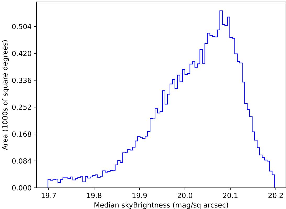
ddf_loaded_fl1_v3.4_10yrs WFD i band: Median skyBrightness
