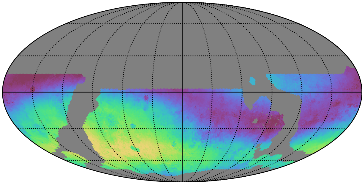
ddf_loaded_fl1_v3.4_10yrs WFD g band: Median skyBrightness
