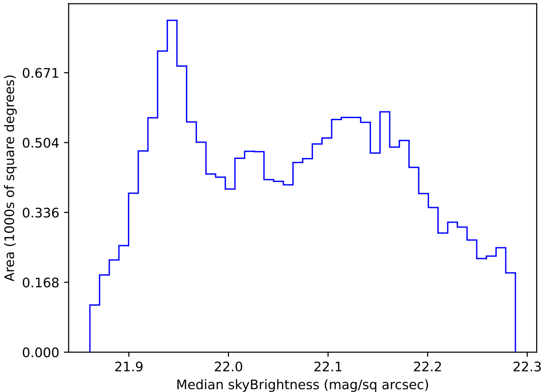
ddf_loaded_fl1_v3.4_10yrs WFD g band: Median skyBrightness
