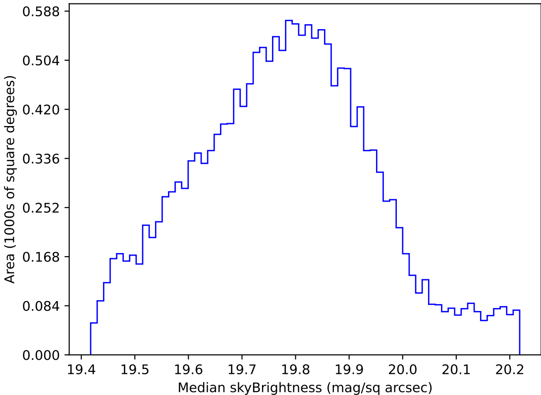
ddf_loaded_fl1_v3.4_10yrs WFD all bands: Median skyBrightness
