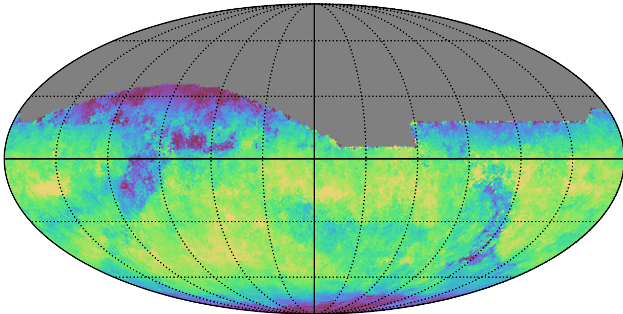
ddf_loaded_fl1_v3.4_10yrs All sky z band: Median skyBrightness
