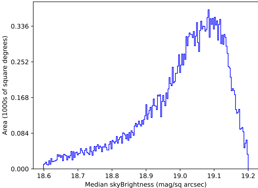
ddf_loaded_fl1_v3.4_10yrs All sky z band: Median skyBrightness
