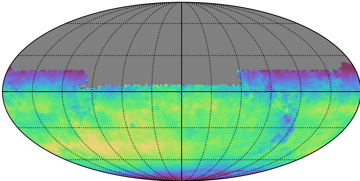
ddf_loaded_fl1_v3.4_10yrs All sky y band: Median skyBrightness
