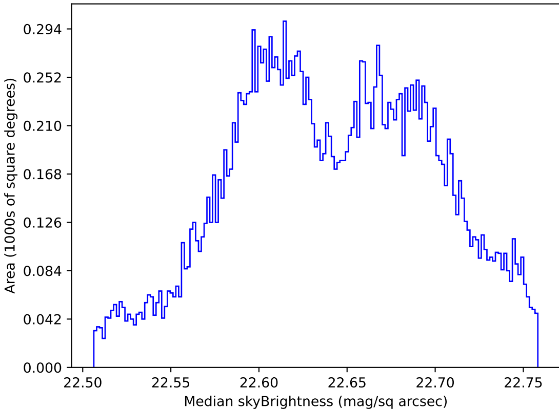
ddf_loaded_fl1_v3.4_10yrs All sky u band: Median skyBrightness
