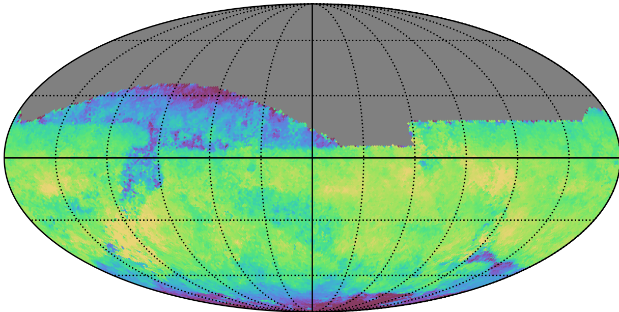
ddf_loaded_fl1_v3.4_10yrs All sky i band: Median skyBrightness
