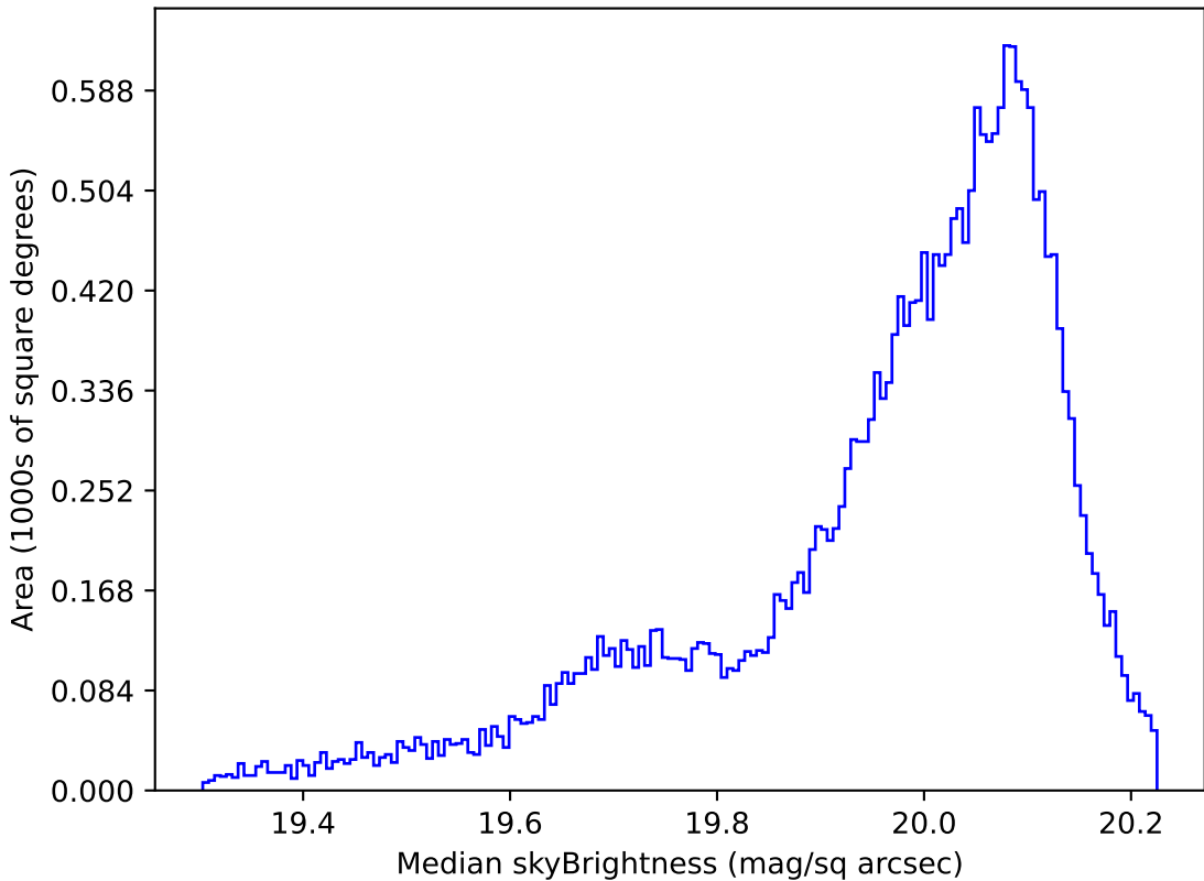
ddf_loaded_fl1_v3.4_10yrs All sky i band: Median skyBrightness
