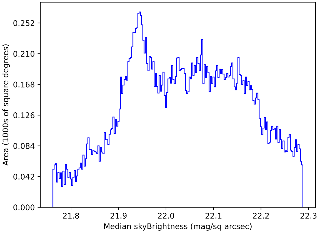
ddf_loaded_fl1_v3.4_10yrs All sky g band: Median skyBrightness
