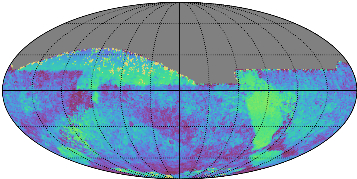
ddf_loaded_fl1_v3.4_10yrs All sky all bands: Median skyBrightness
