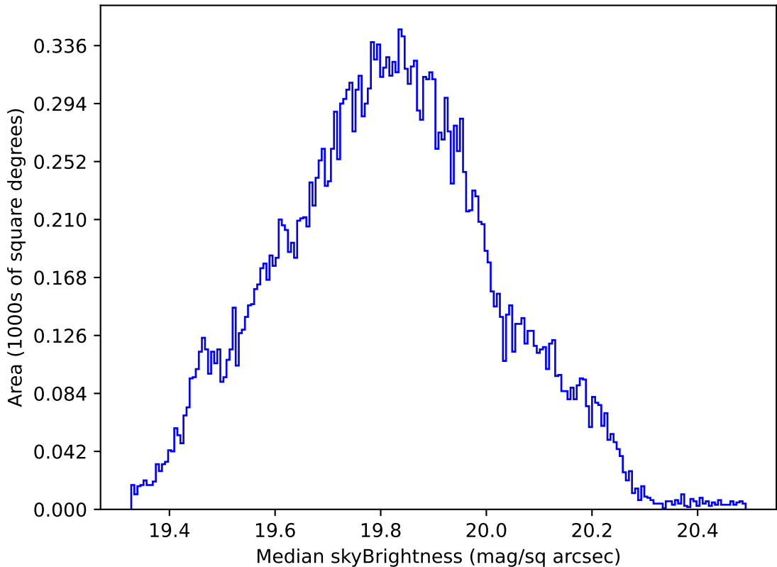
ddf_loaded_fl1_v3.4_10yrs All sky all bands: Median skyBrightness
