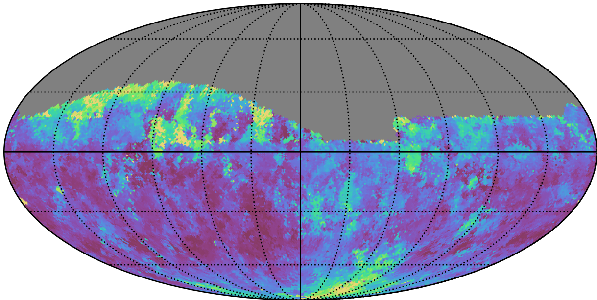
ddf_loaded_fl1_v3.4_10yrs Yr 1 z band: Median seeingGeom
