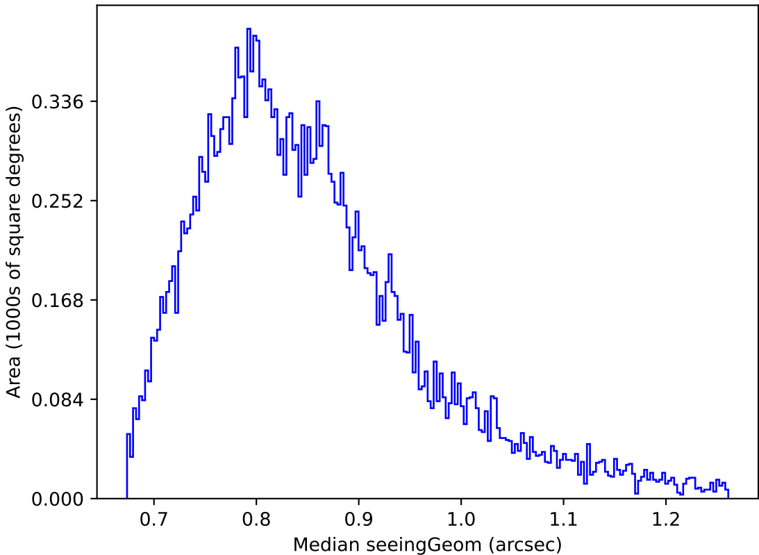
ddf_loaded_fl1_v3.4_10yrs Yr 1 z band: Median seeingGeom
