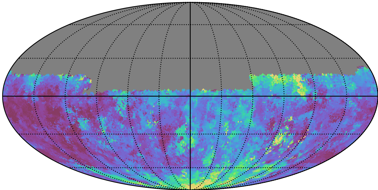
ddf_loaded_fl1_v3.4_10yrs Yr 1 u band: Median seeingGeom
