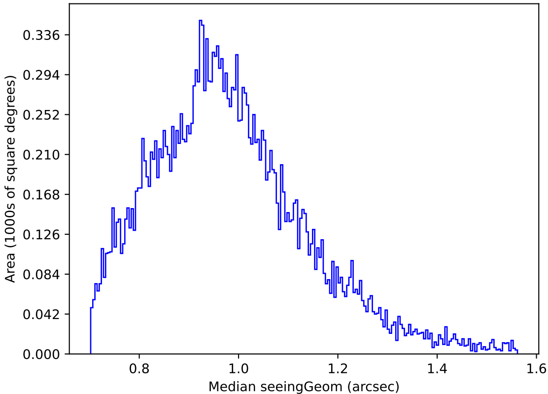
ddf_loaded_fl1_v3.4_10yrs Yr 1 u band: Median seeingGeom
